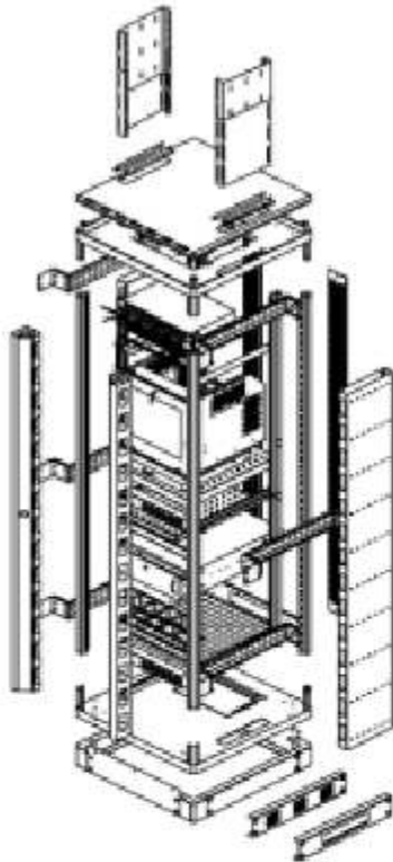
Explode View
